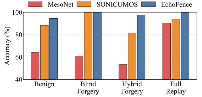
Fig. 7: Overall performance of EchoFence compared to two baselines: MesoNet and SONICUMOS.
